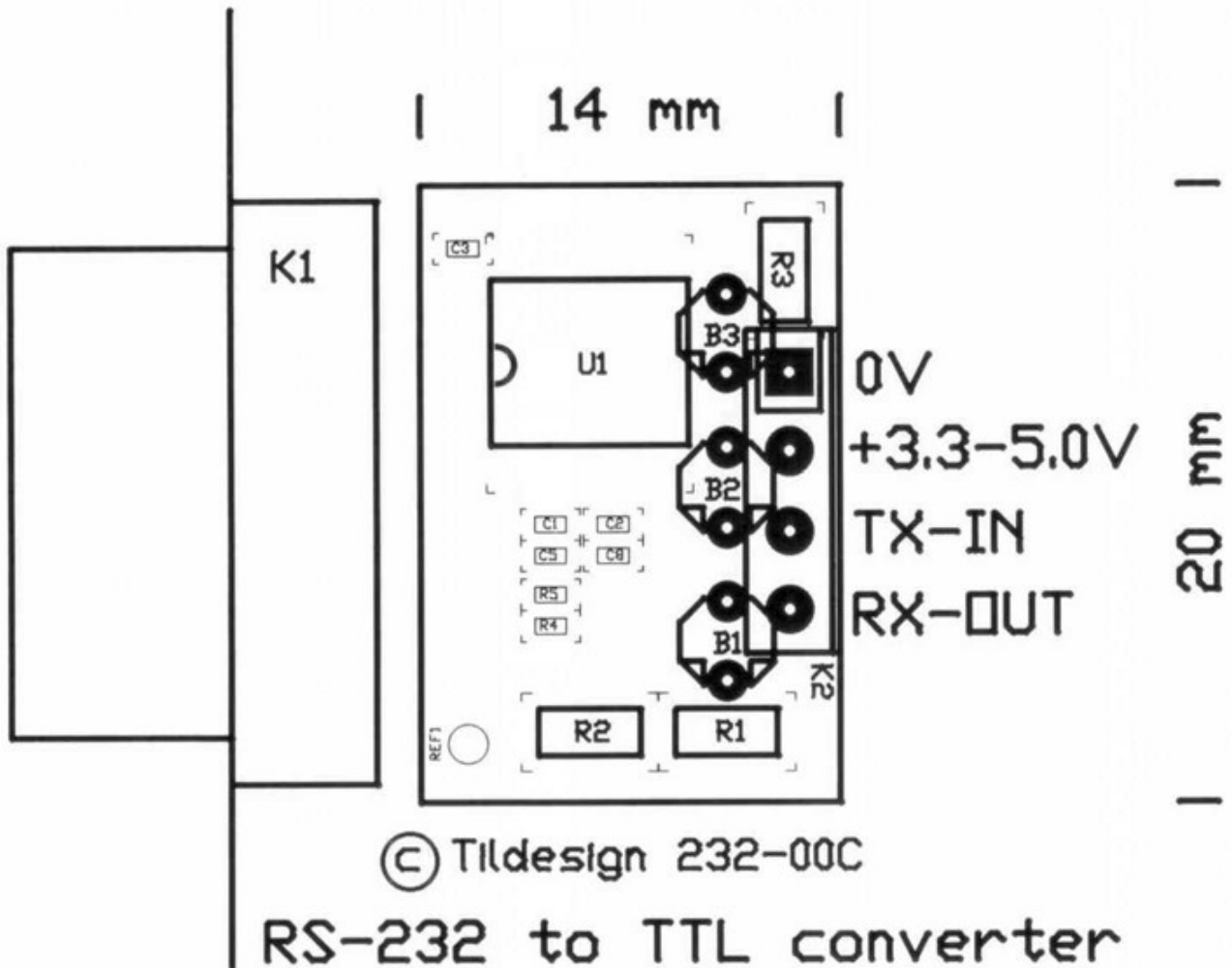
Component layout
